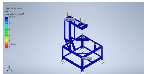
Gambar 6. Safety Factor
