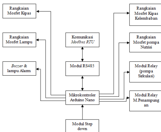
Gambar 19. Blok Board Control
