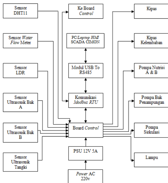
Gambar 18. Blok Diagram Control Smart Green House
