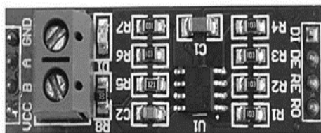
Gambar 6. Modul RS-485 (Santoso, 2015)
