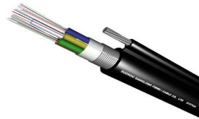
Gambar 9 (a) Kabel Aerial
