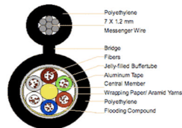
Gambar 9(b) Penampang Kabel Aerial
