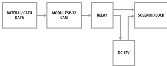
Gbr. 2 Blok Diagram Hardware
